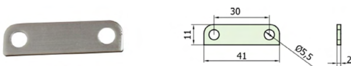
PWB375SP – Peg Stay Bracket Spacer
