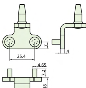
PWS375THPB – Peg Stay “Through-Hole-Pin” for Top and Side Hung Windows
