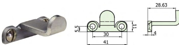
PWB375VRST – Peg Stay Rest Bracket
