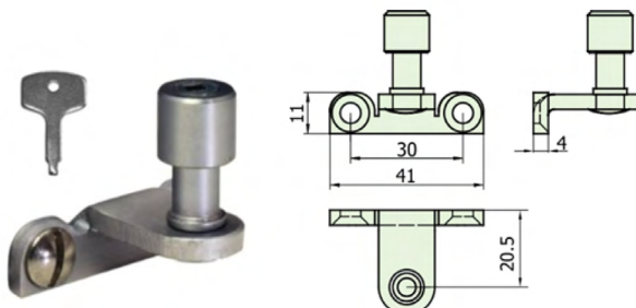
PWB375VLPB – Key Locking Peg Stay Pin Bracket
