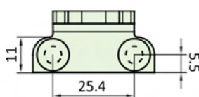
PWS375FB – Peg Stay Fixing Bracket (3 sizes)
