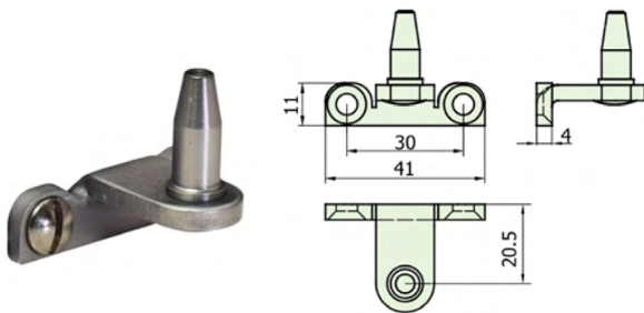
PWB375VPB – Peg Stay “Through-Hole-Pin” Bracket
